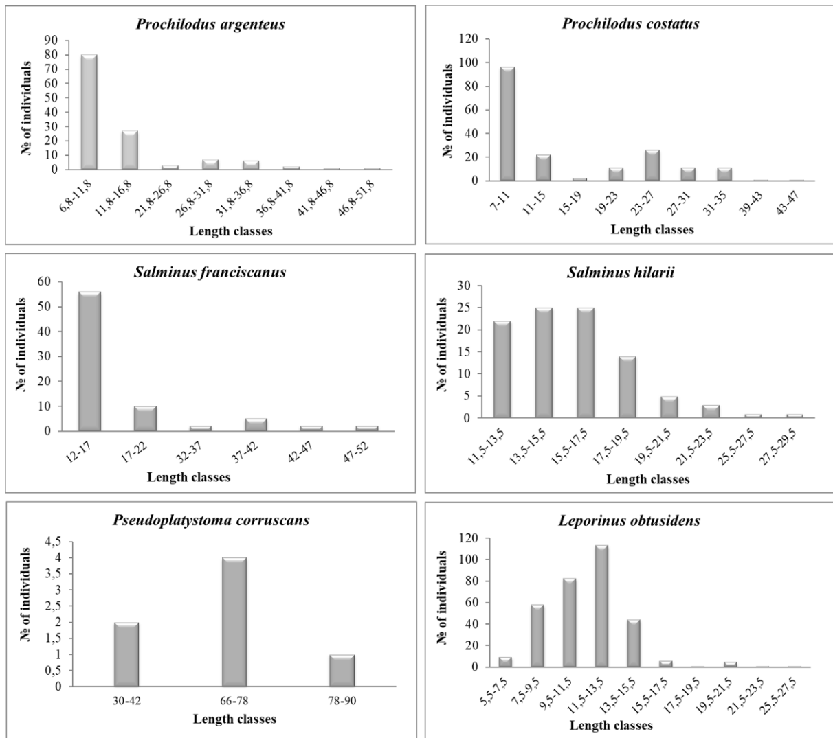
FIGURE 2: Length classes of six species of migratory fishes that showed recruitment in the Jequitai River basin, Minas Gerais, Brazil.
